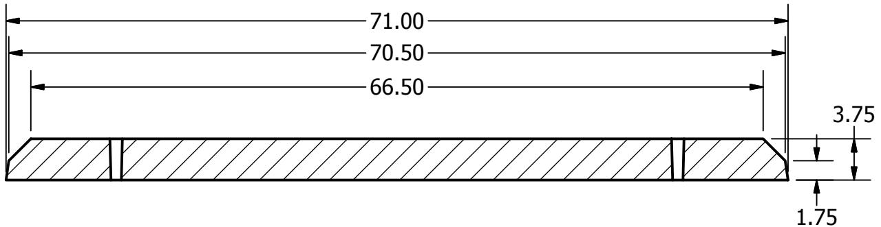
SECTION B-B SCALE 1 / 12
